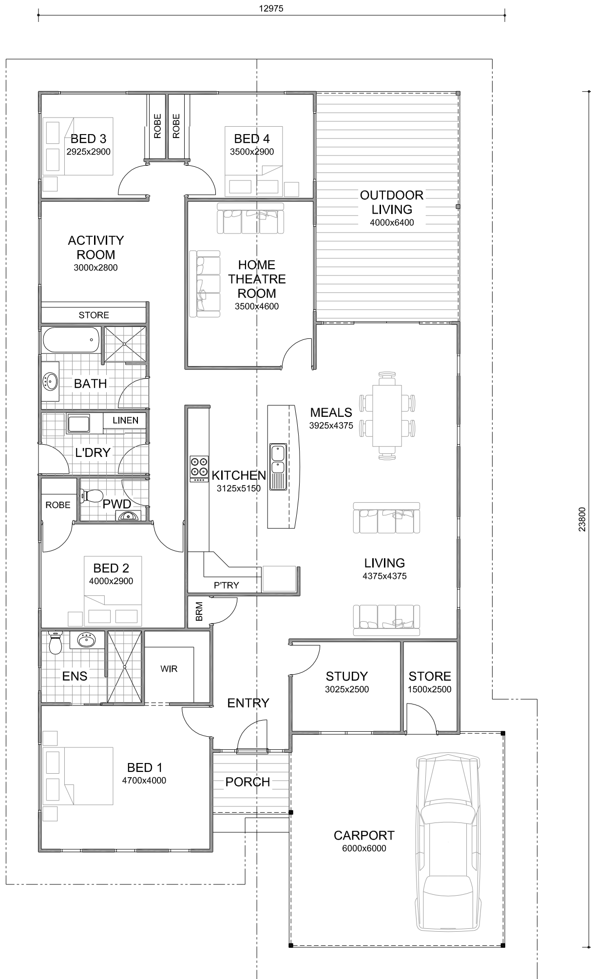
FLOOR PLAN
