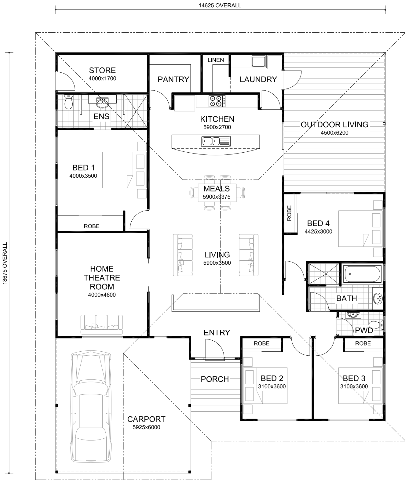
FLOOR PLAN
