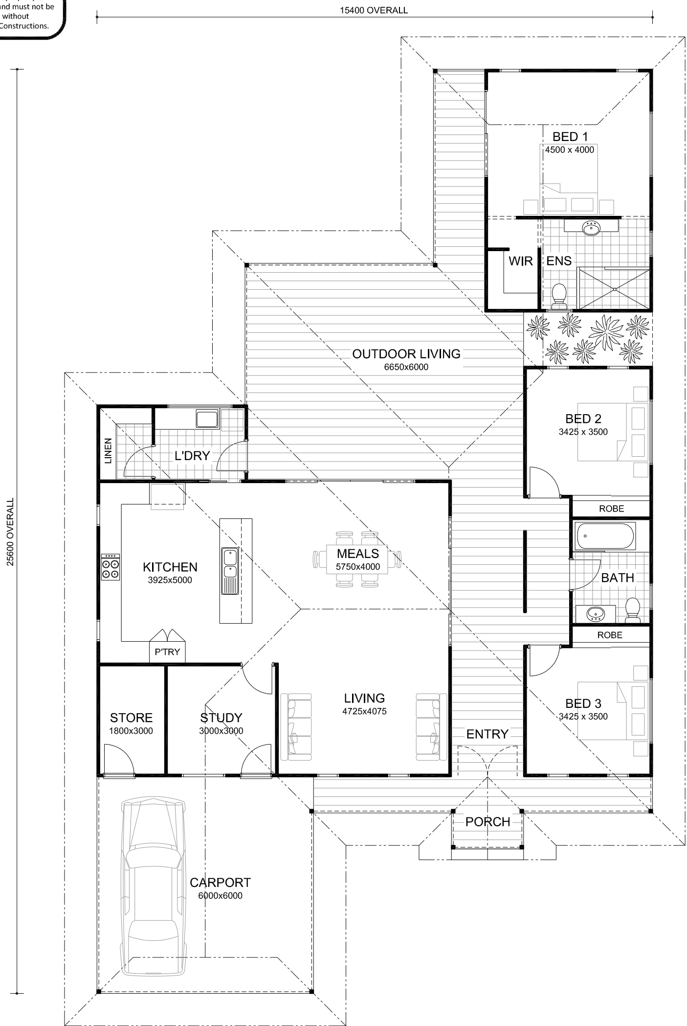
FLOOR PLAN
